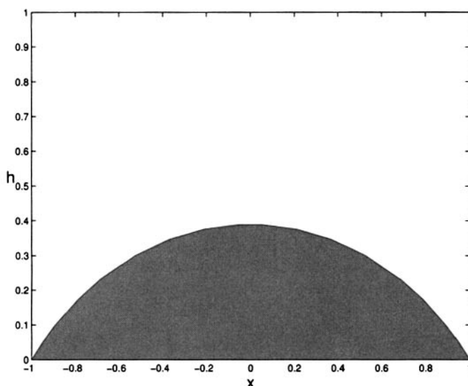
Figure 12.14. Water droplet BVP solved by bvp4c .
