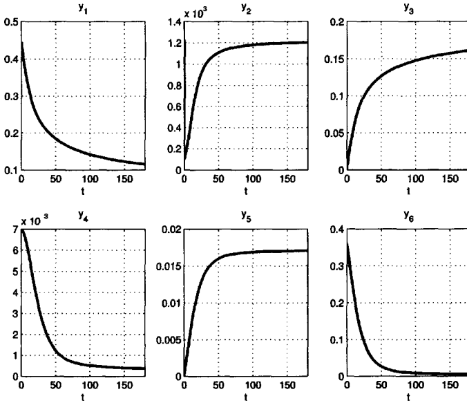
Figure 12.13. DAE solution components from chemakzo in Listing 12.7.
