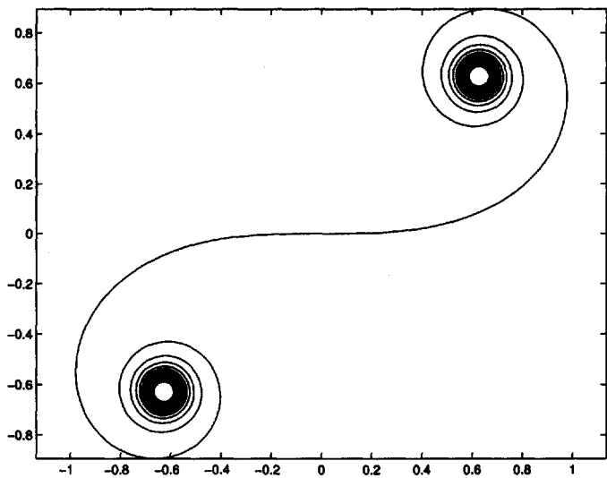
Figure 12.2. Fresnel spiral.
