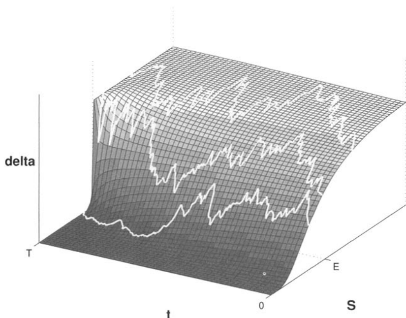
Figure 22.7. Black-Scholes delta picture from bsdelta.
