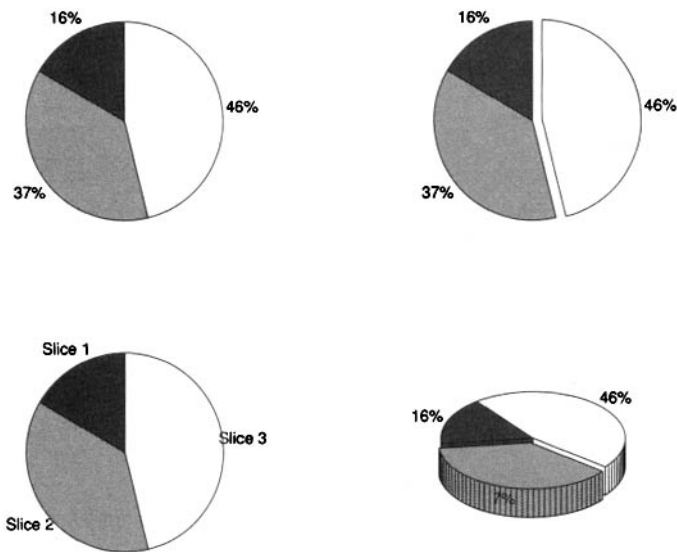
Figure 8.25. Pie charts.
