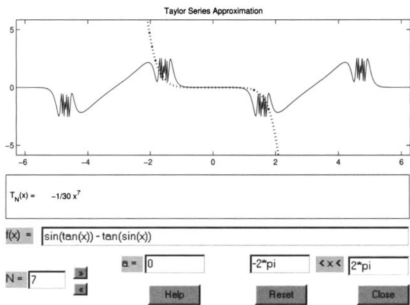
Figure 19.1. taylortool window.
