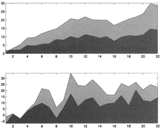
Figure 8.26. Area graphs.
