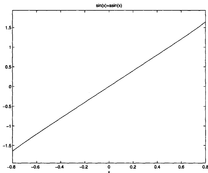
Figure 19.2. \sin(x) + \arcsin(x)
