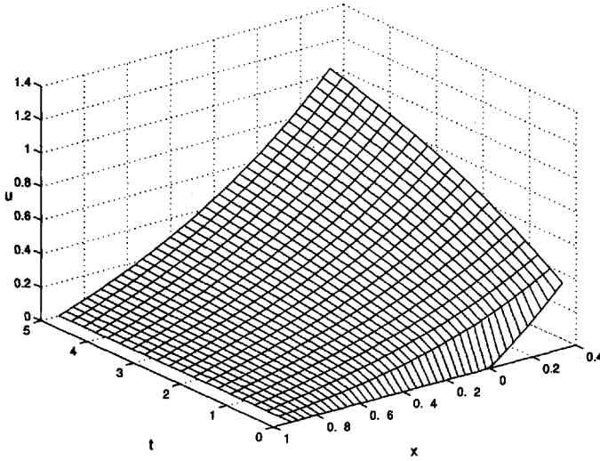
Figure 12.19. Black-Scholes solution with pdepe.
