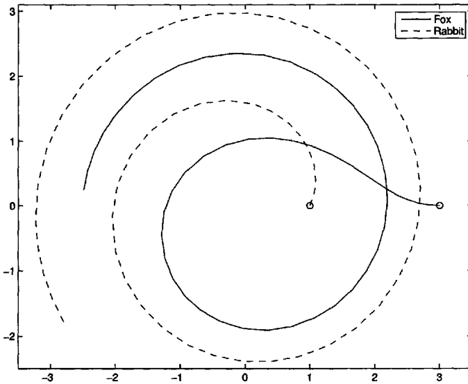
Figure 12.8. Pursuit example.
