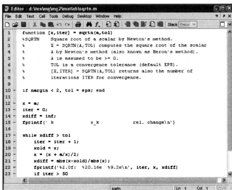
Figure 7.2. MATLAB Editor/Debugger.
