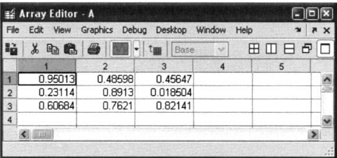
Figure 2.3. Array Editor.
