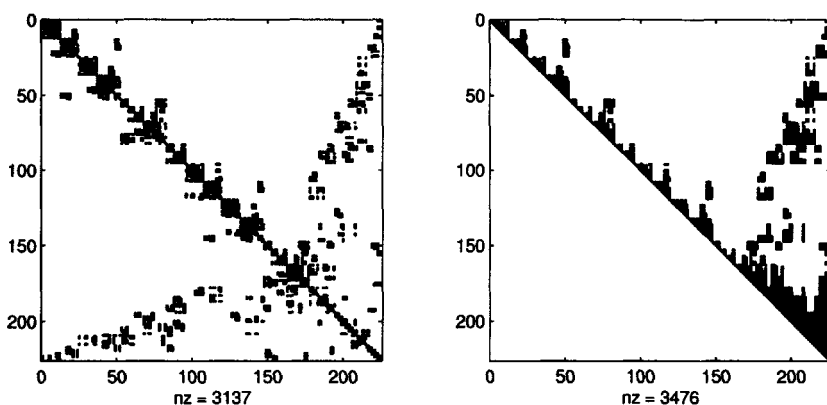
Figure 15.3. Wathen matrix (left) and its Cholesky factor (right) with symmetric minimum degree ordering (symamd).
