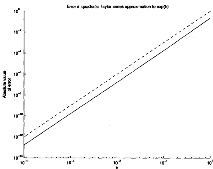
Figure 8.3. loglog example.
