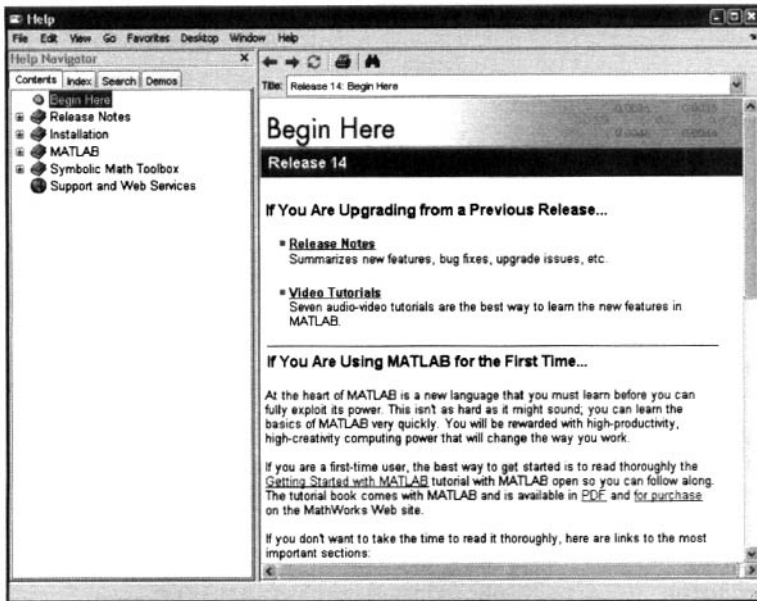
Figure 2.1. Help browser.
