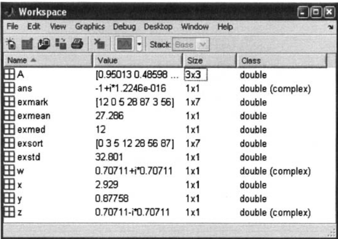
Figure 2.2. Workspace browser.
