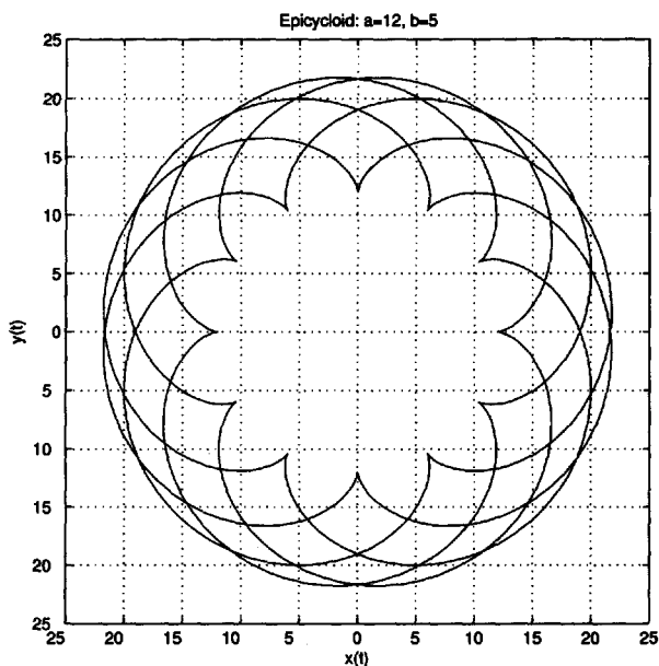
Figure 8.6. Epicycloid example.
