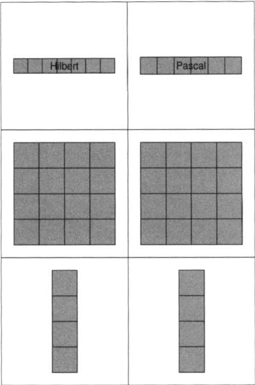
Figure 18.2. cellplot(testmat) .
